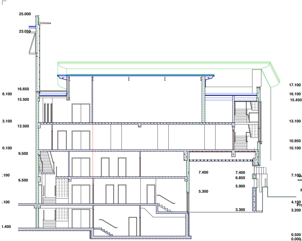
Section E5-E5
